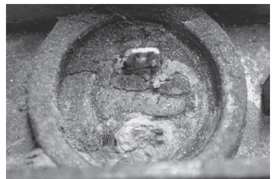
The lower terminal on this lamp became so badly corroded that it broke off.
