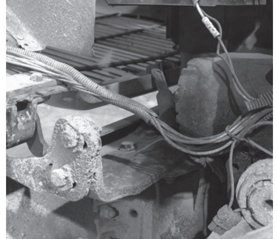
If wiring is installed where it will be subject to repeated flexing such as around doors, hatches and moving equipment, it is subject to special stress and wear.
