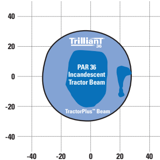
IsoCandela Footprint
