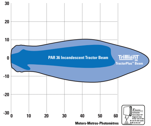
IsoLux Footprint
