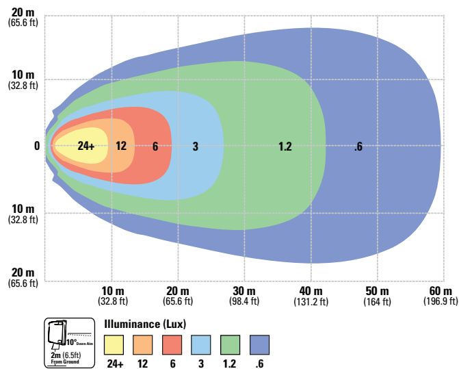
1800 Lumen Near Pattern
