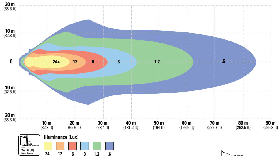
1800 Lumen Far Pattern
