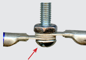
LONGER NECK ELIMINATES OBSTRUCTION FROM TUBING TO ENSURE 100% SURFACE CONTACT
