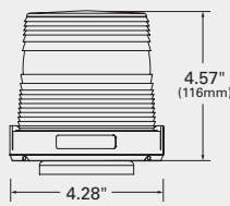
Magnetic Mount
