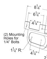
"Z" MOUNTING BRACKET FOR OVAL LAMPS
