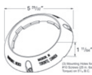
SURFACE MOUNT BRACKET FOR 4" LED LAMPS
