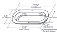
THEFT-RESISTANT MOUNTING FLANGE FOR OVAL LAMPS
